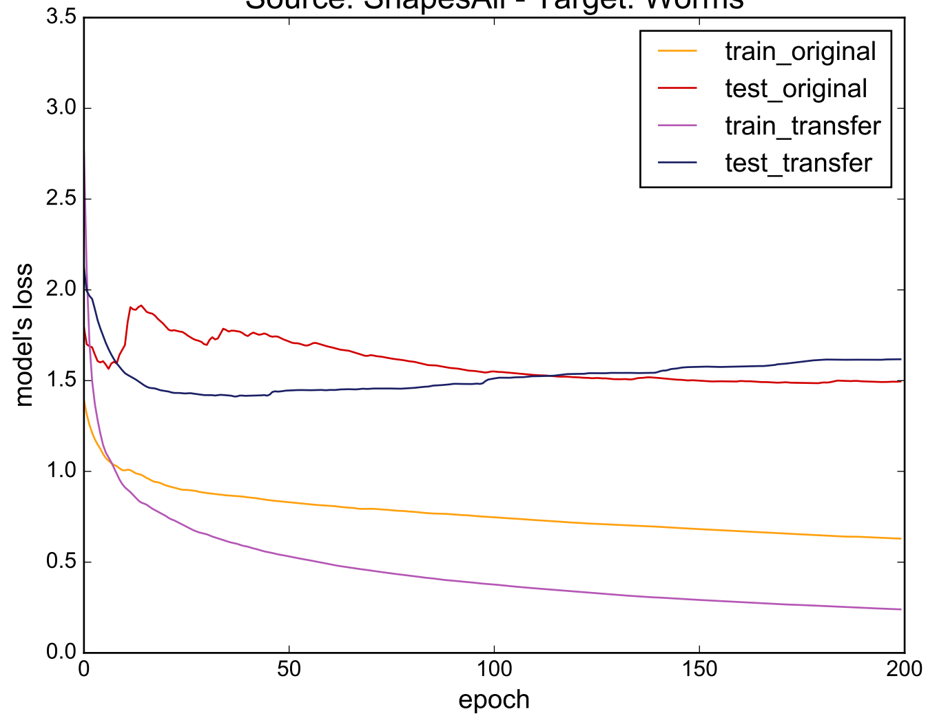
Source: ShapesAll - Target: Worms
