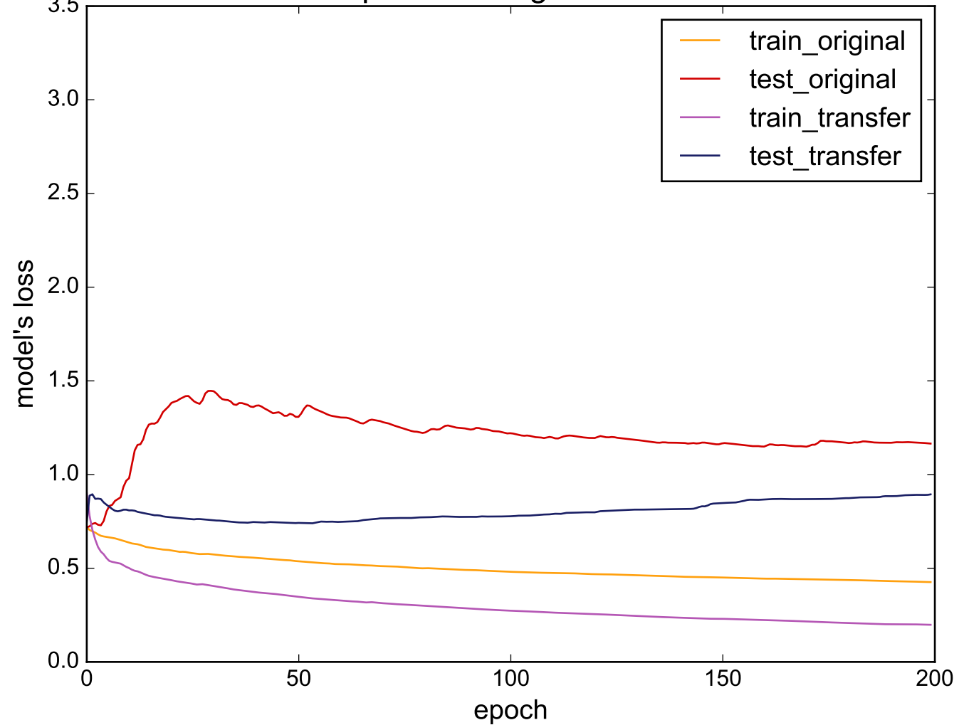
Source: ShapesAll - Target: WormsTwoClass
