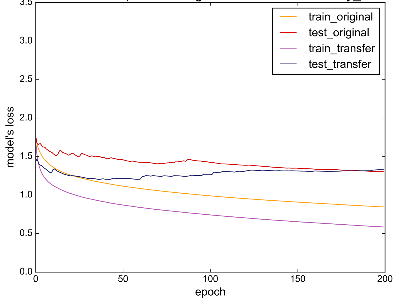
Source: ShapesAll - Target: uWaveGestureLibrary_Y
