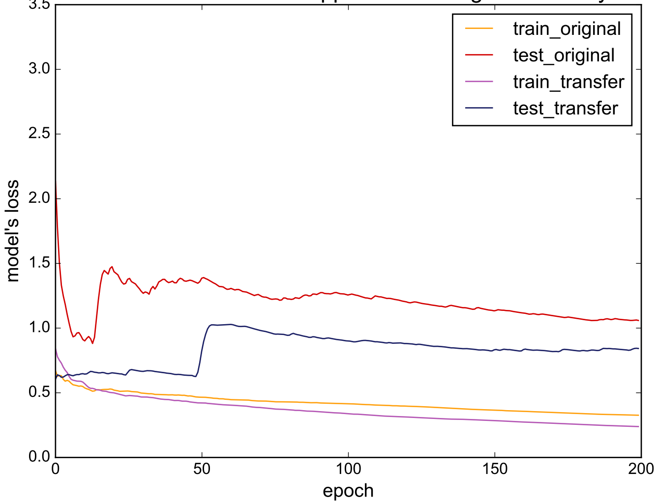
Source: SmallKitchenAppliances - Target: BeetleFly
