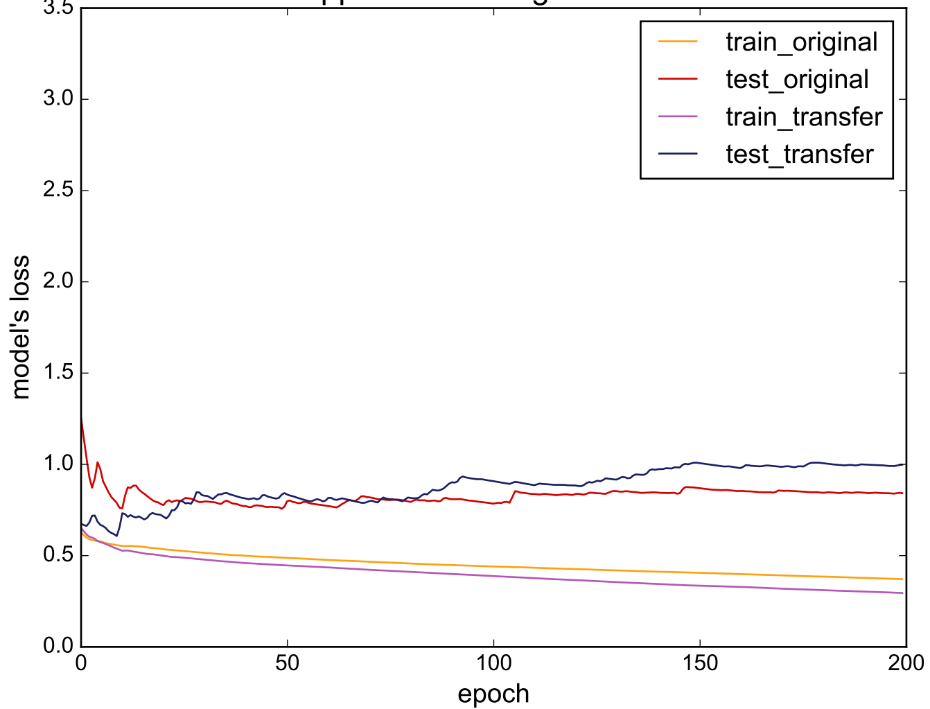
Source: SmallKitchenAppliances - Target: DistalPhalanxOutlineCorrect
