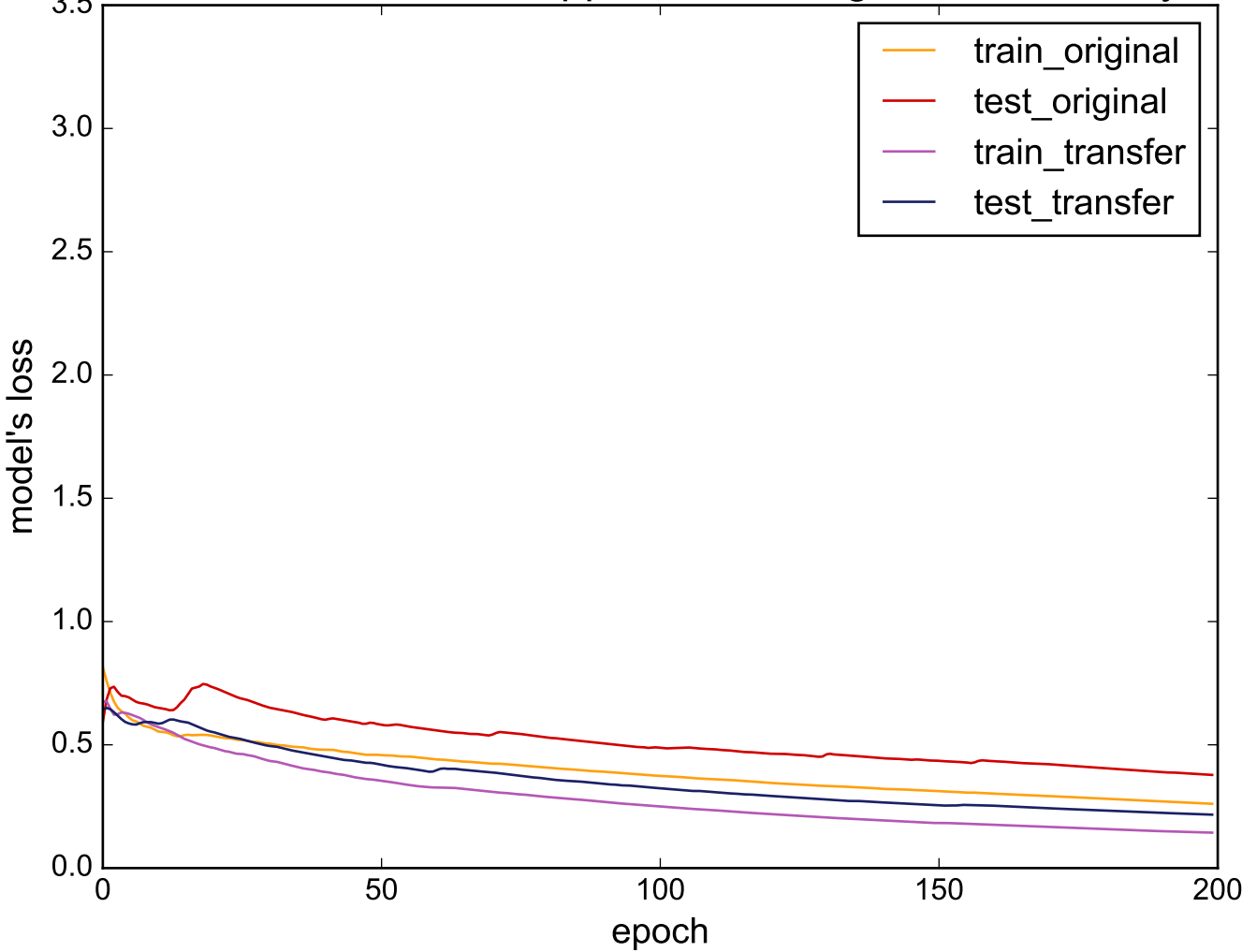
Source: SmallKitchenAppliances - Target: ECGFiveDays
