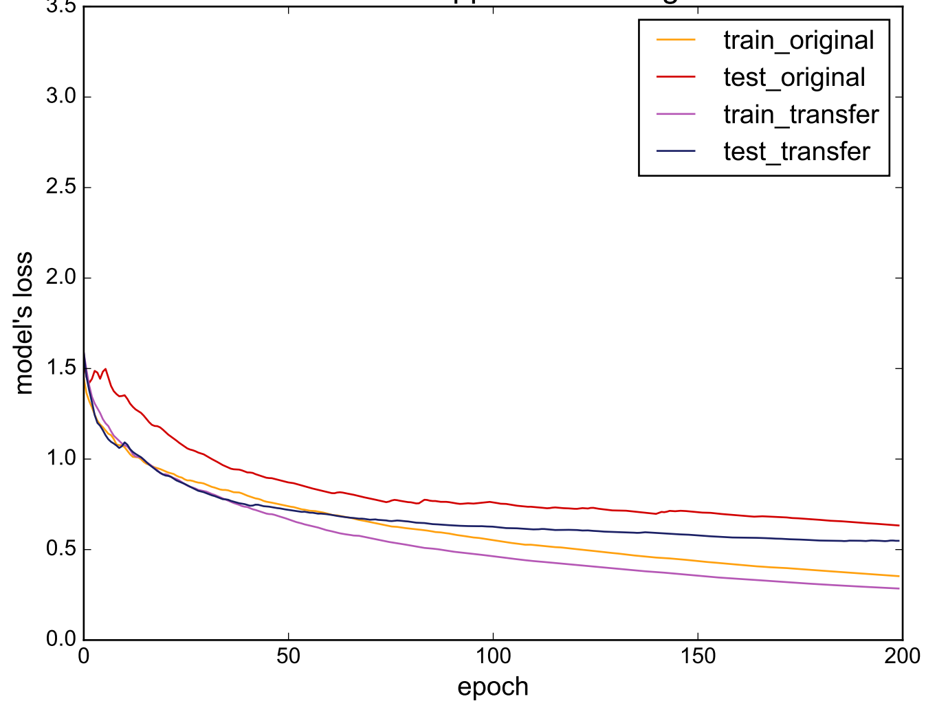
Source: SmallKitchenAppliances - Target: FaceFour
