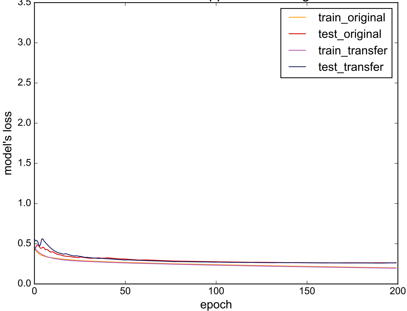
Source: SmallKitchenAppliances - Target: FordA
