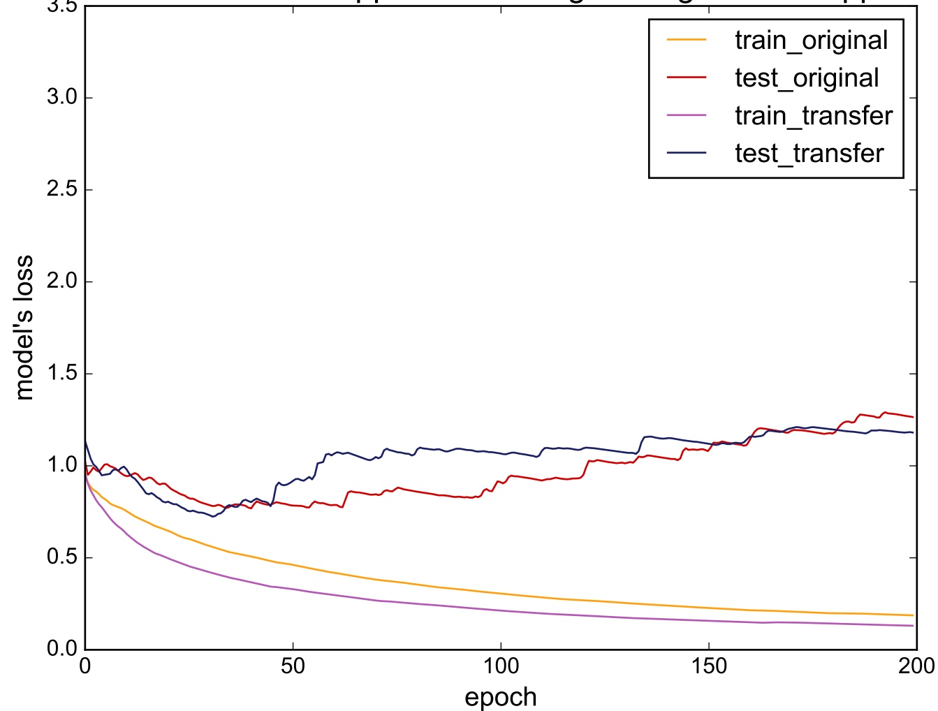
Source: SmallKitchenAppliances - Target: LargeKitchenAppliances
