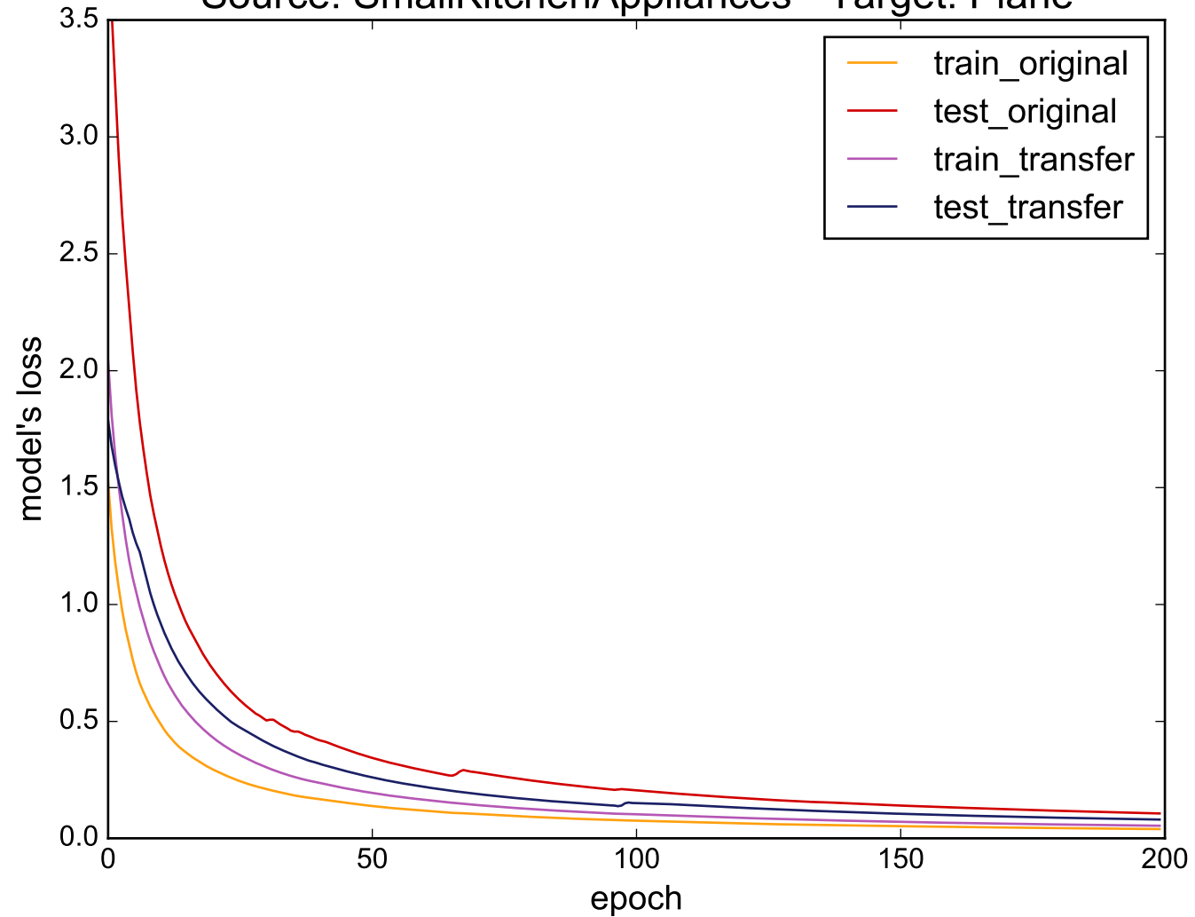
Source: SmallKitchenAppliances - Target: Plane
