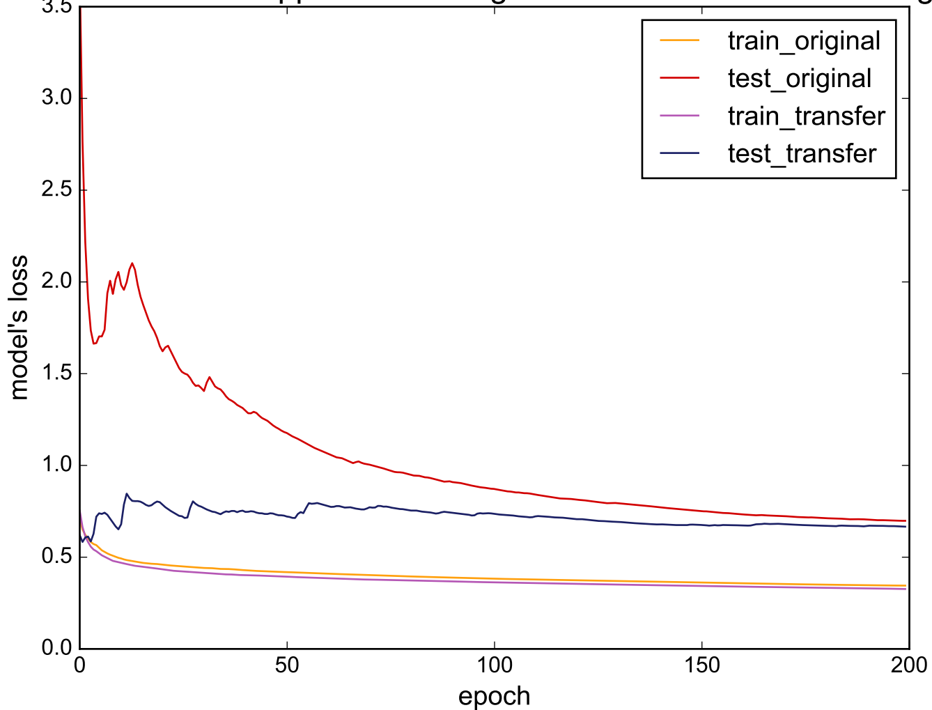
Source: SmallKitchenAppliances - Target: ProximalPhalanxOutlineAgeGroup
