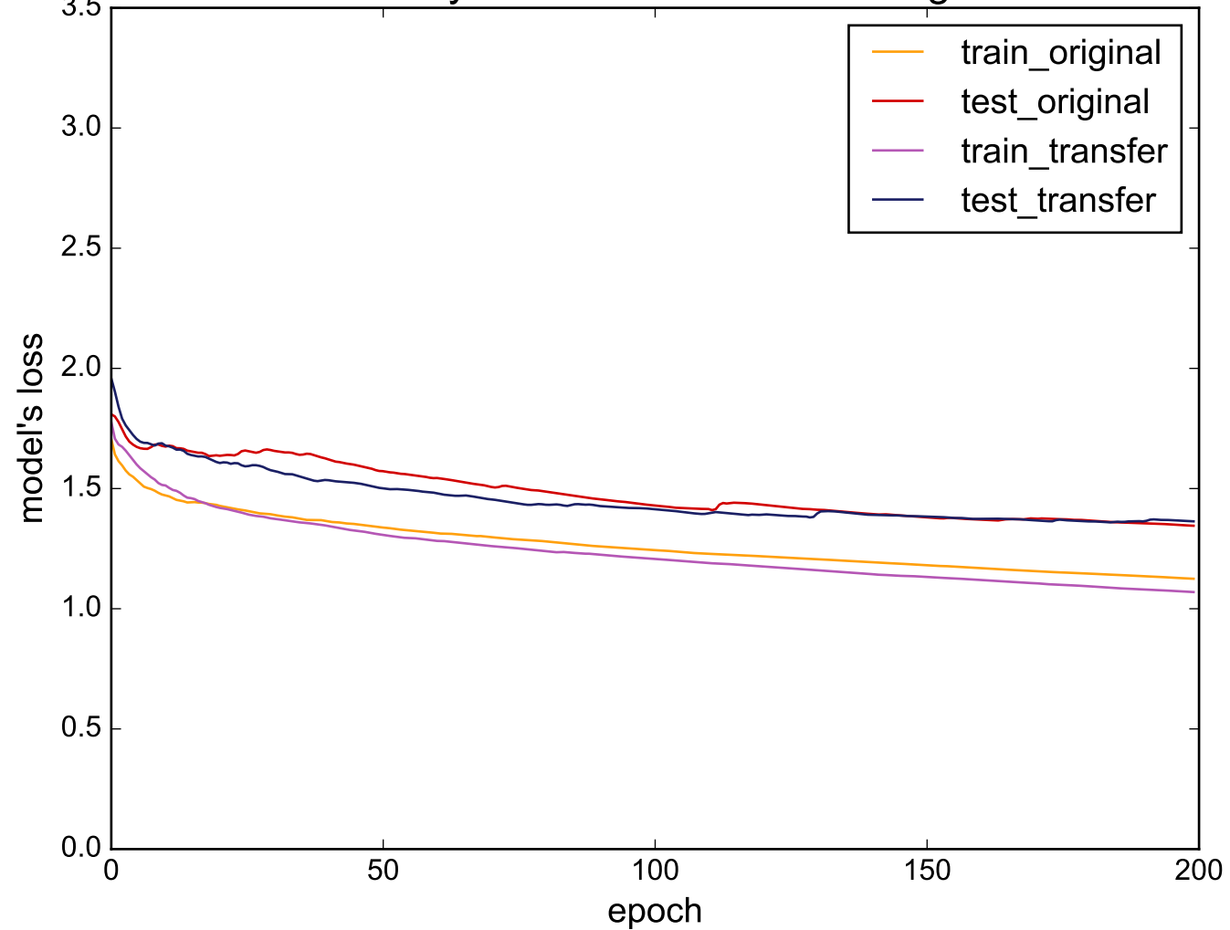
Source: SonyAIBORobotSurface - Target: Beef
