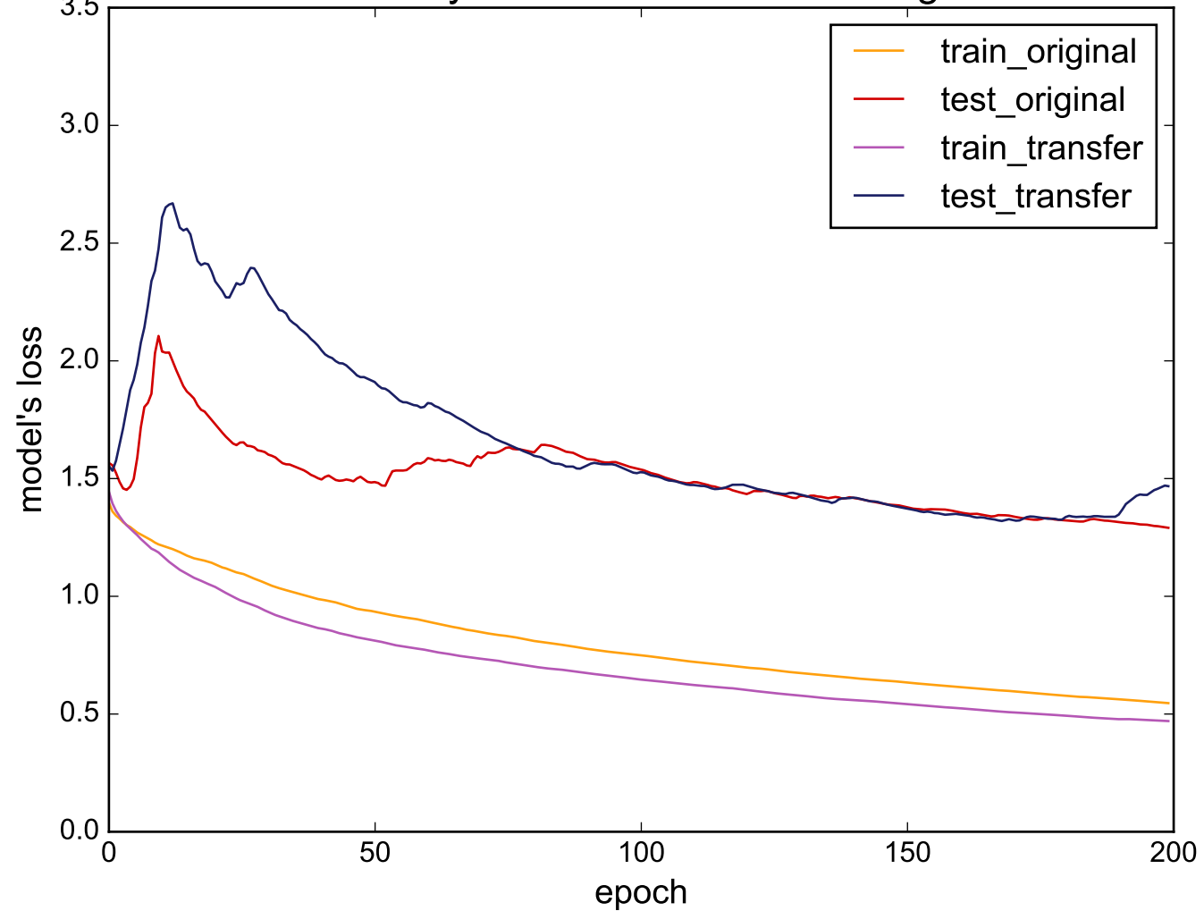
Source: SonyAIBORobotSurface - Target: Car
