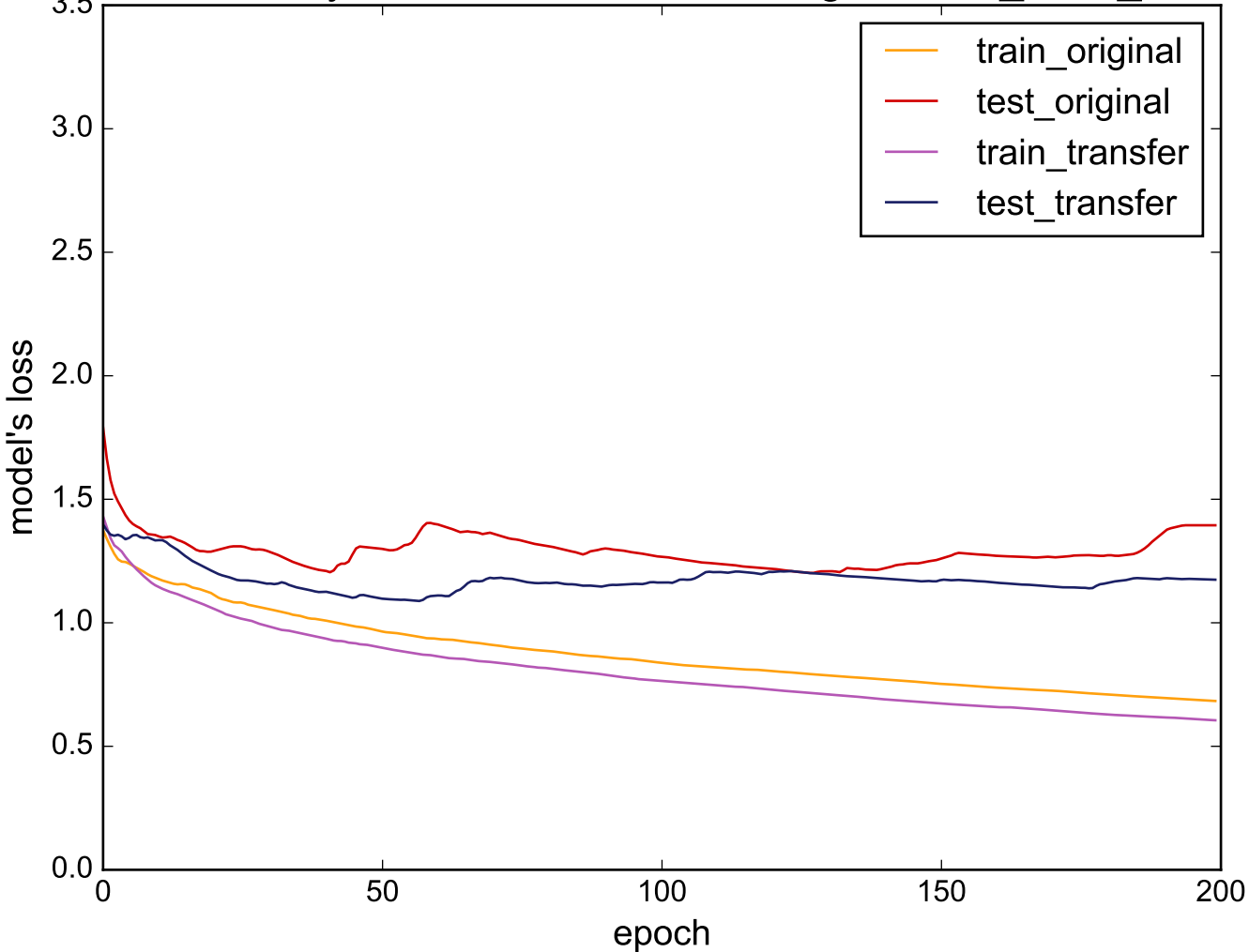
Source: SonyAIBORobotSurface - Target: CinC_ECG_torso
