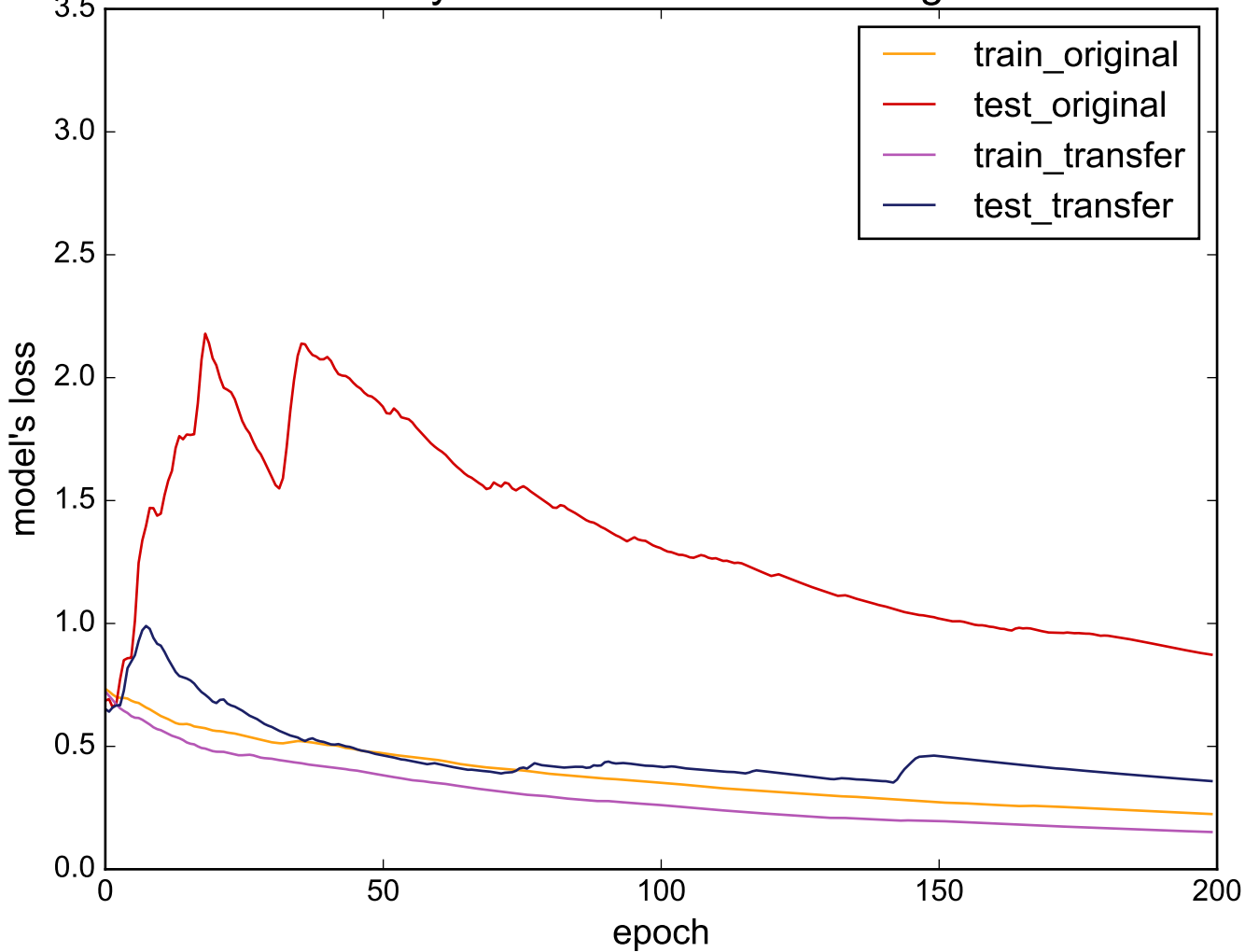
Source: SonyAIBORobotSurface - Target: Coffee
