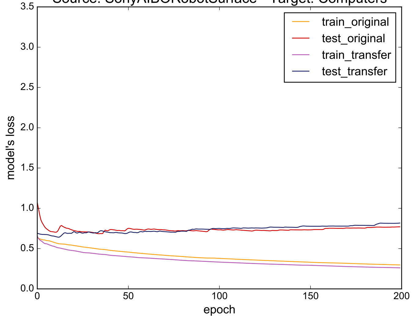
Source: SonyAIBORobotSurface - Target: Computers
