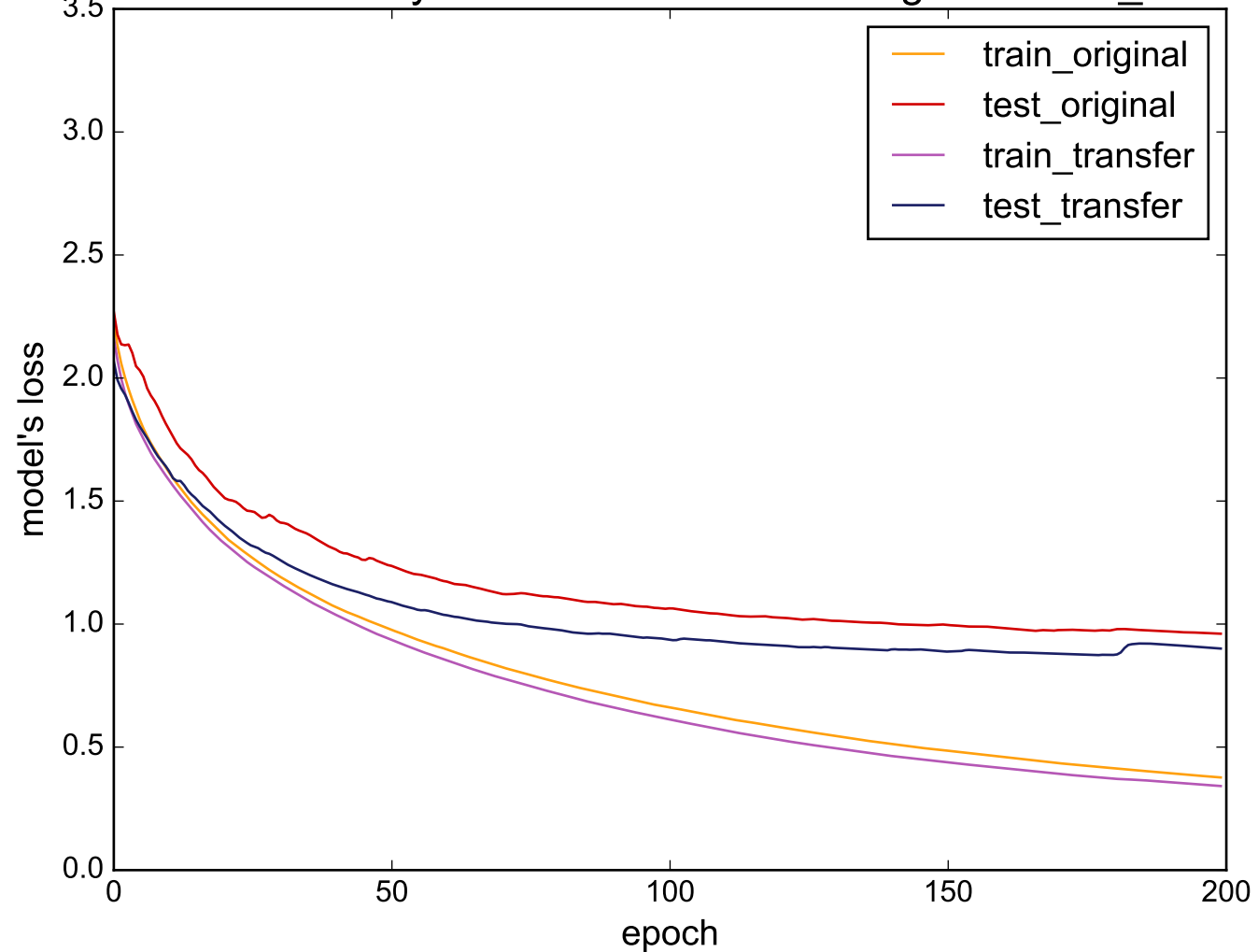
Source: SonyAIBORobotSurface - Target: Cricket_Z
