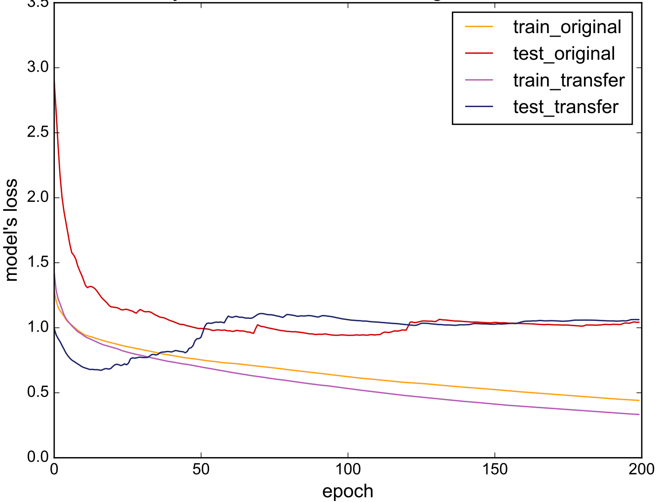
Source: SonyAIBORobotSurface - Target: DistalPhalanxTW
