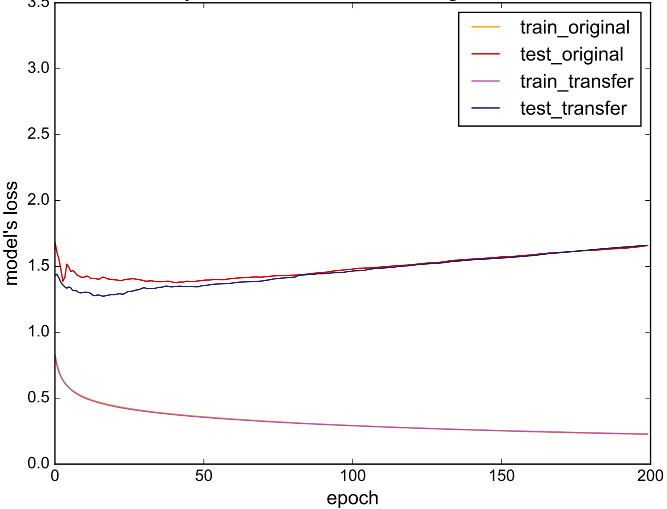
Source: SonyAIBORobotSurface - Target: ElectricDevices
