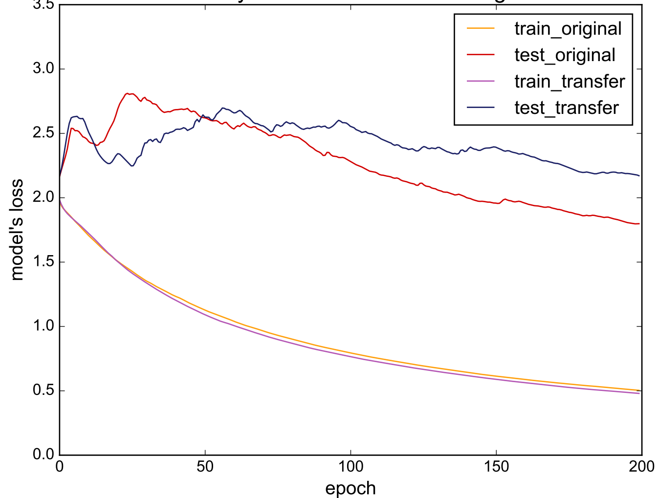
Source: SonyAIBORobotSurface - Target: FISH
