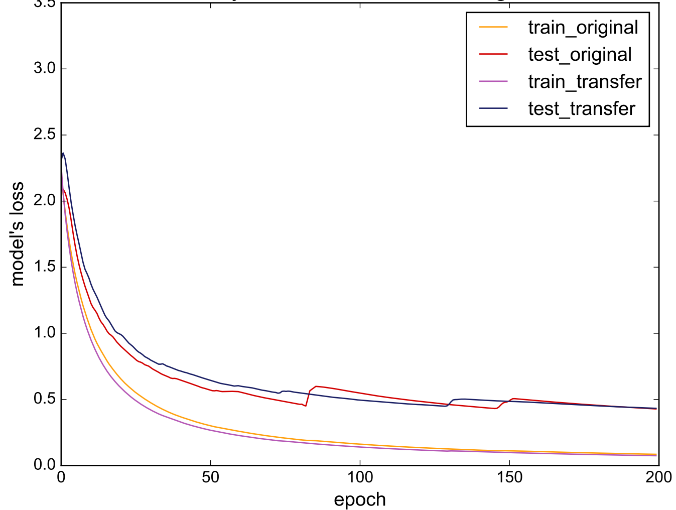
Source: SonyAIBORobotSurface - Target: FaceAll
