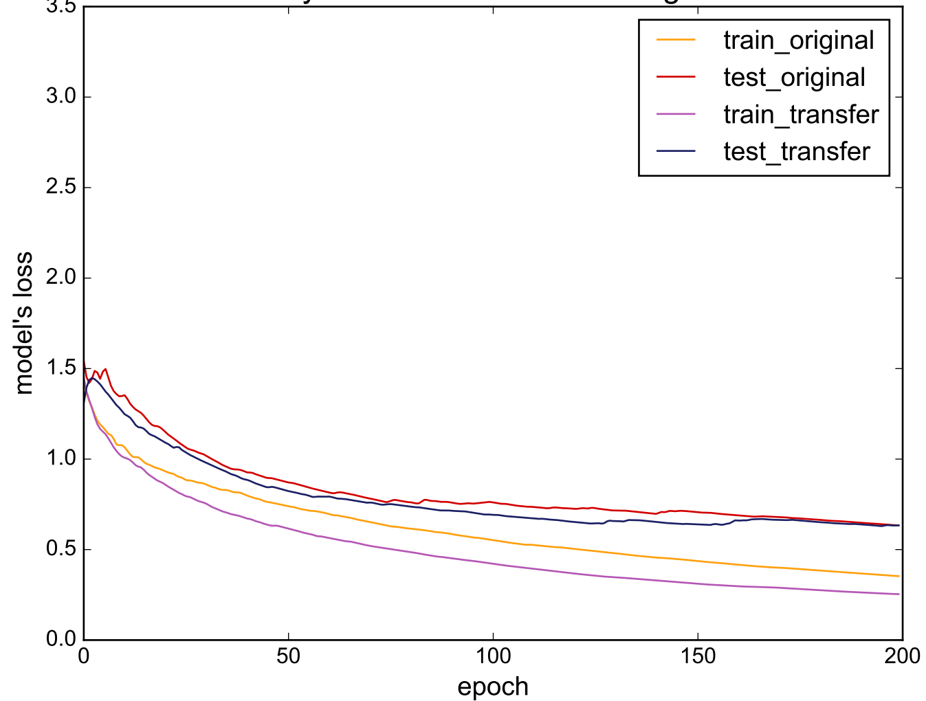
Source: SonyAIBORobotSurface - Target: FaceFour
