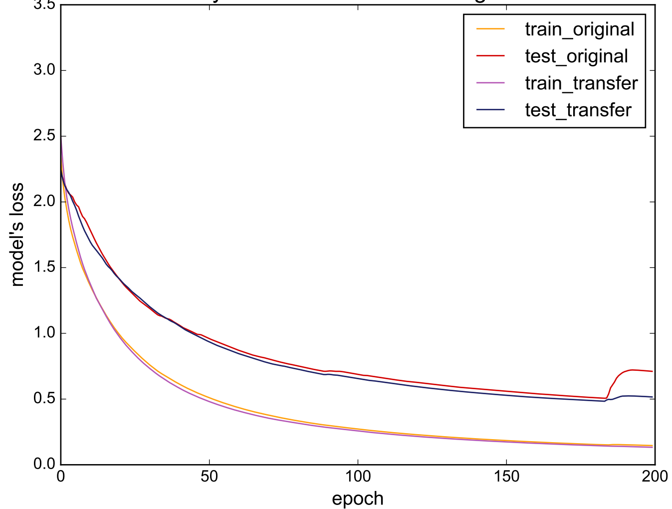
Source: SonyAIBORobotSurface - Target: FacesUCR
