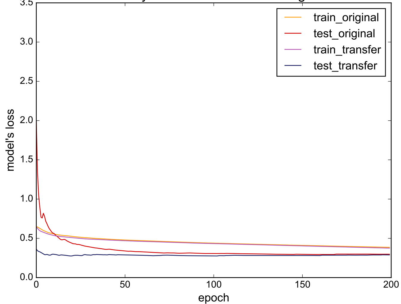
Source: SonyAIBORobotSurface - Target: FordB
