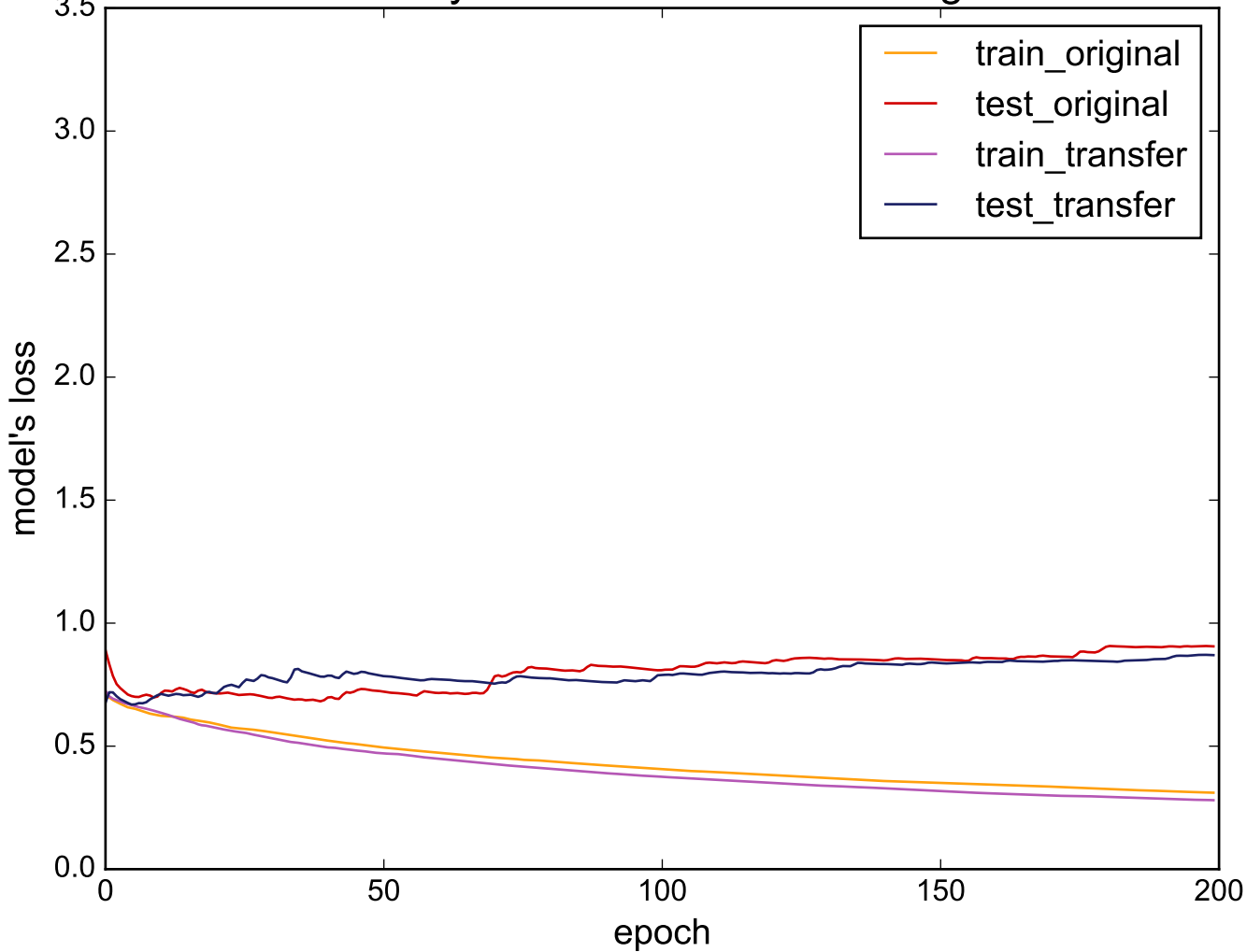
Source: SonyAIBORobotSurface - Target: Ham
