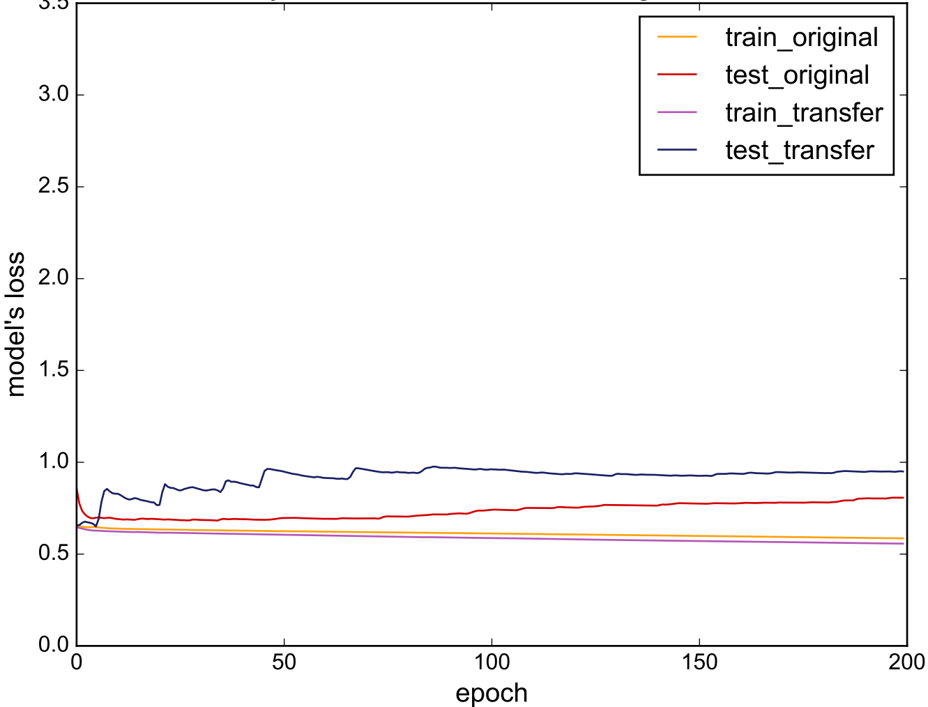
Source: SonyAIBORobotSurface - Target: HandOutlines
