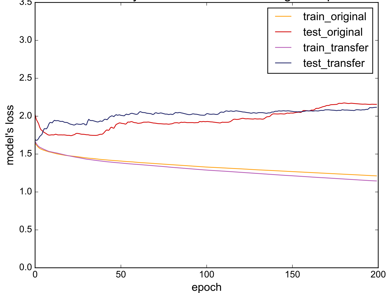
Source: SonyAIBORobotSurface - Target: Haptics
