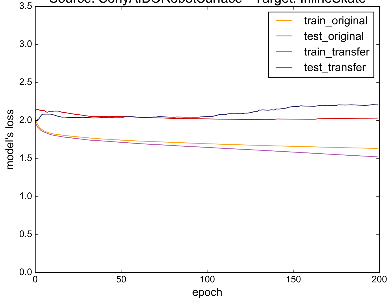
Source: SonyAIBORobotSurface - Target: InlineSkate
