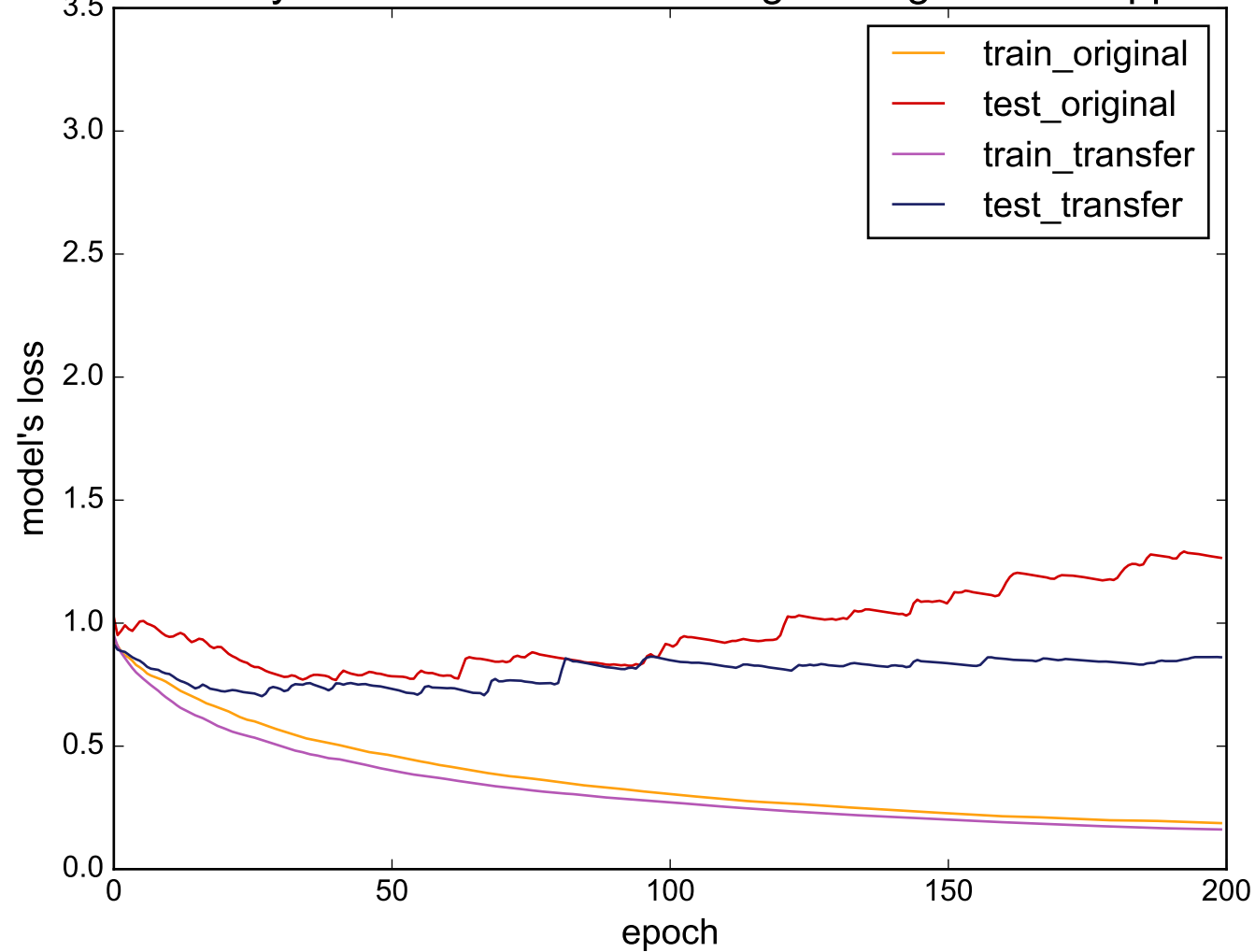
Source: SonyAIBORobotSurface - Target: LargeKitchenAppliances
