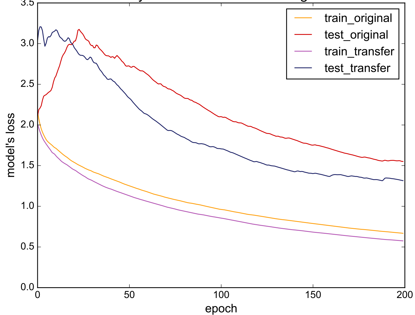
Source: SonyAIBORobotSurface - Target: MALLAT
