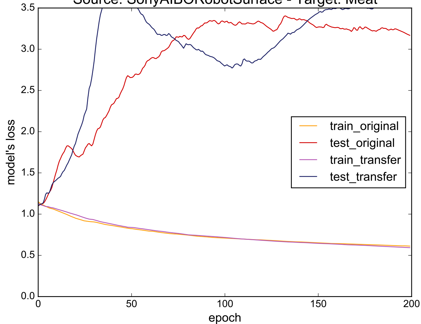
Source: SonyAIBORobotSurface - Target: Meat
