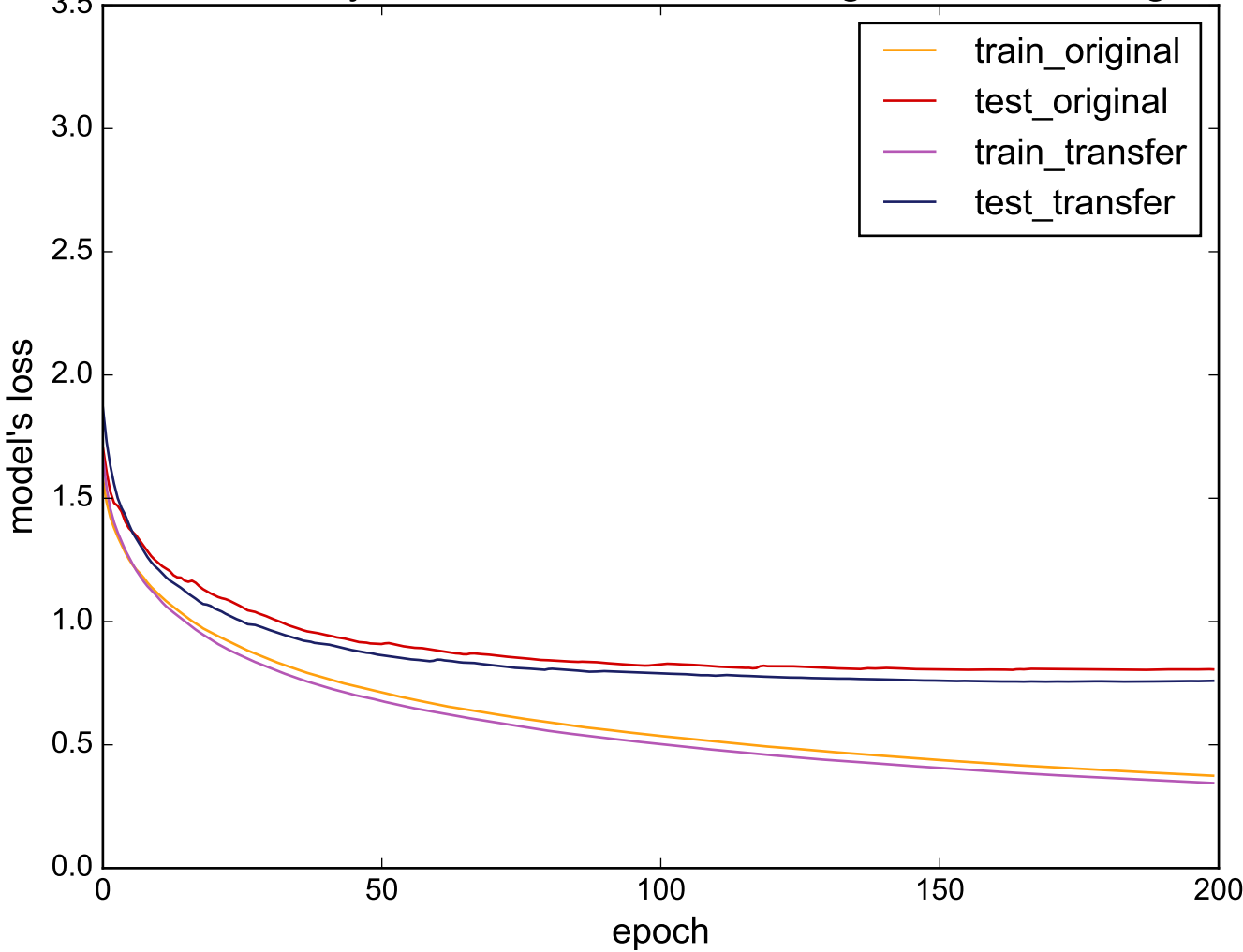
Source: SonyAIBORobotSurface - Target: MedicalImages
