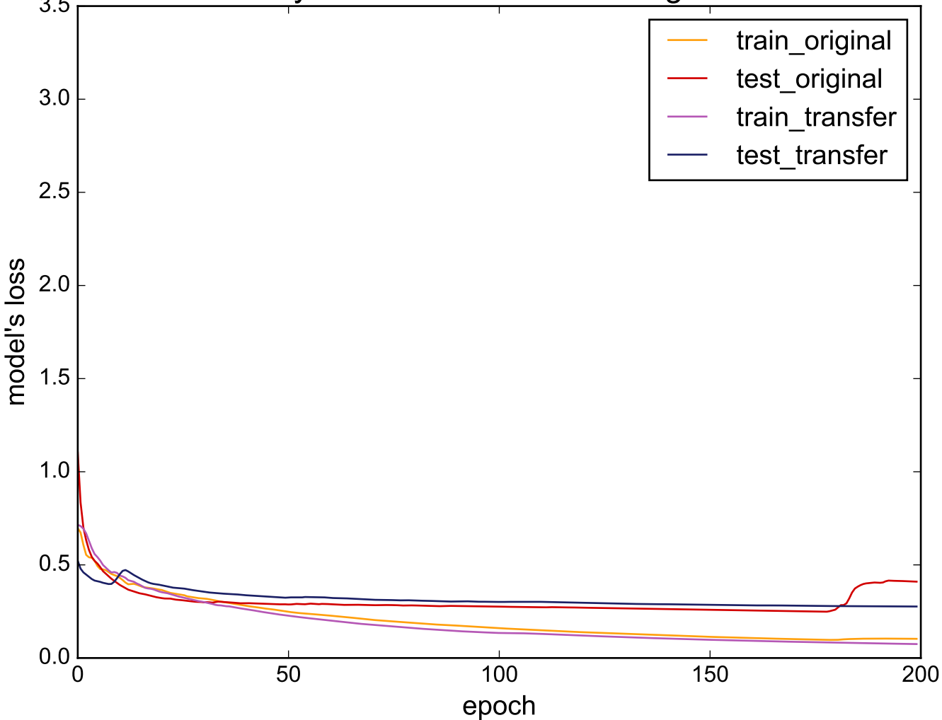
Source: SonyAIBORobotSurface - Target: MoteStrain
