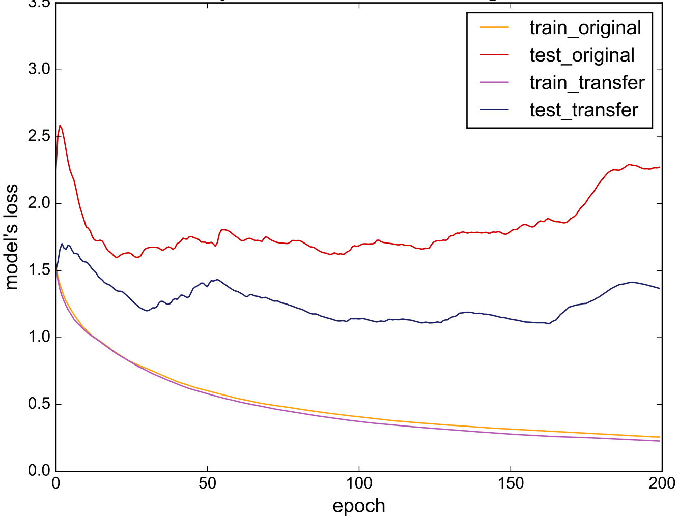
Source: SonyAIBORobotSurface - Target: OSULeaf
