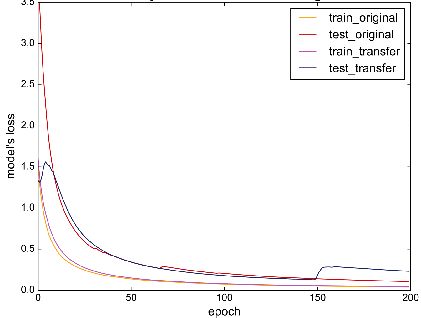
Source: SonyAIBORobotSurface - Target: Plane
