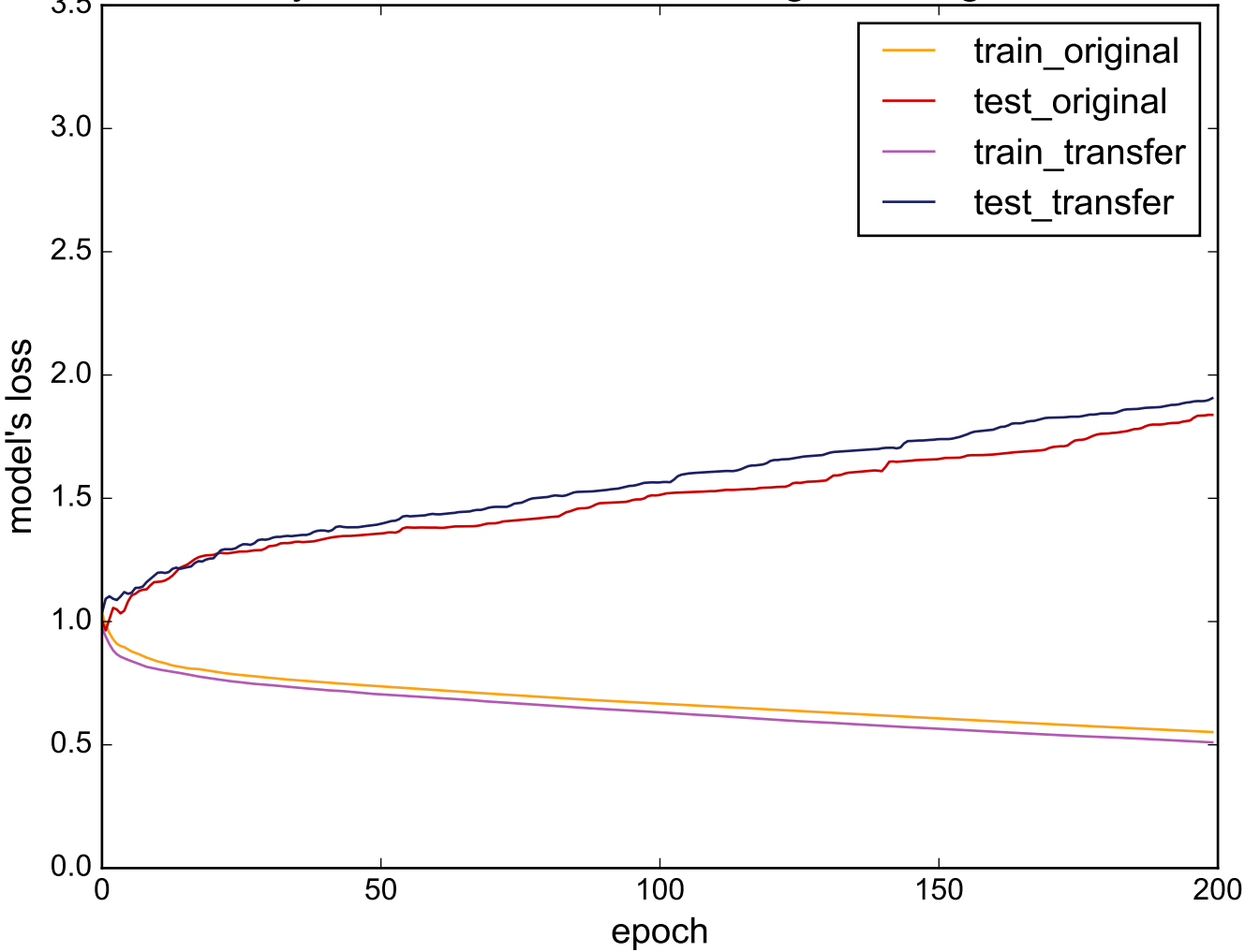
Source: SonyAIBORobotSurface - Target: RefrigerationDevices
