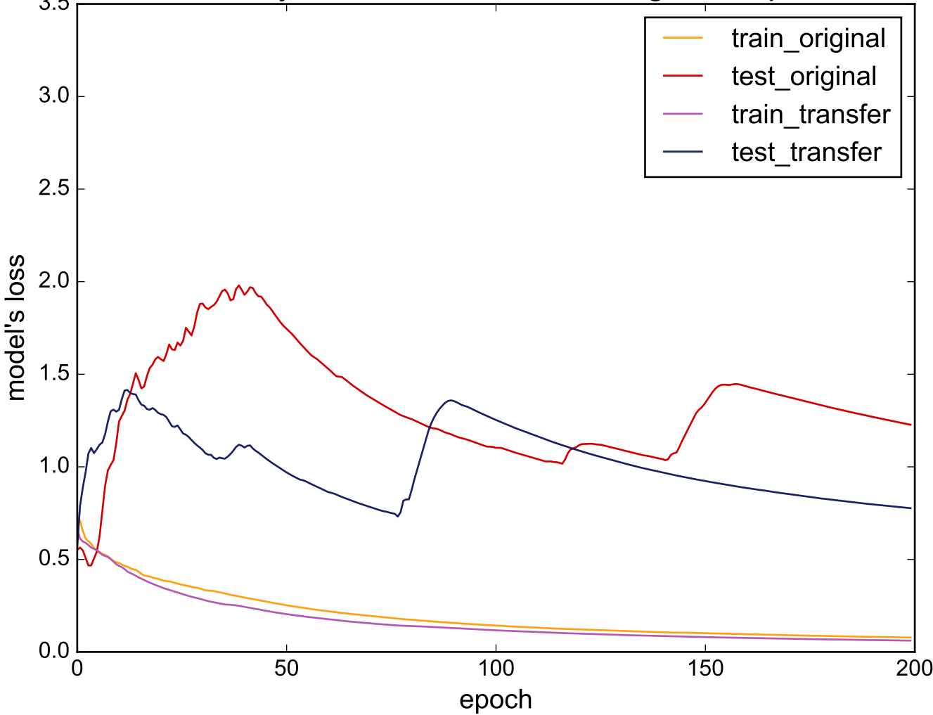
Source: SonyAIBORobotSurface - Target: ShapeletSim
