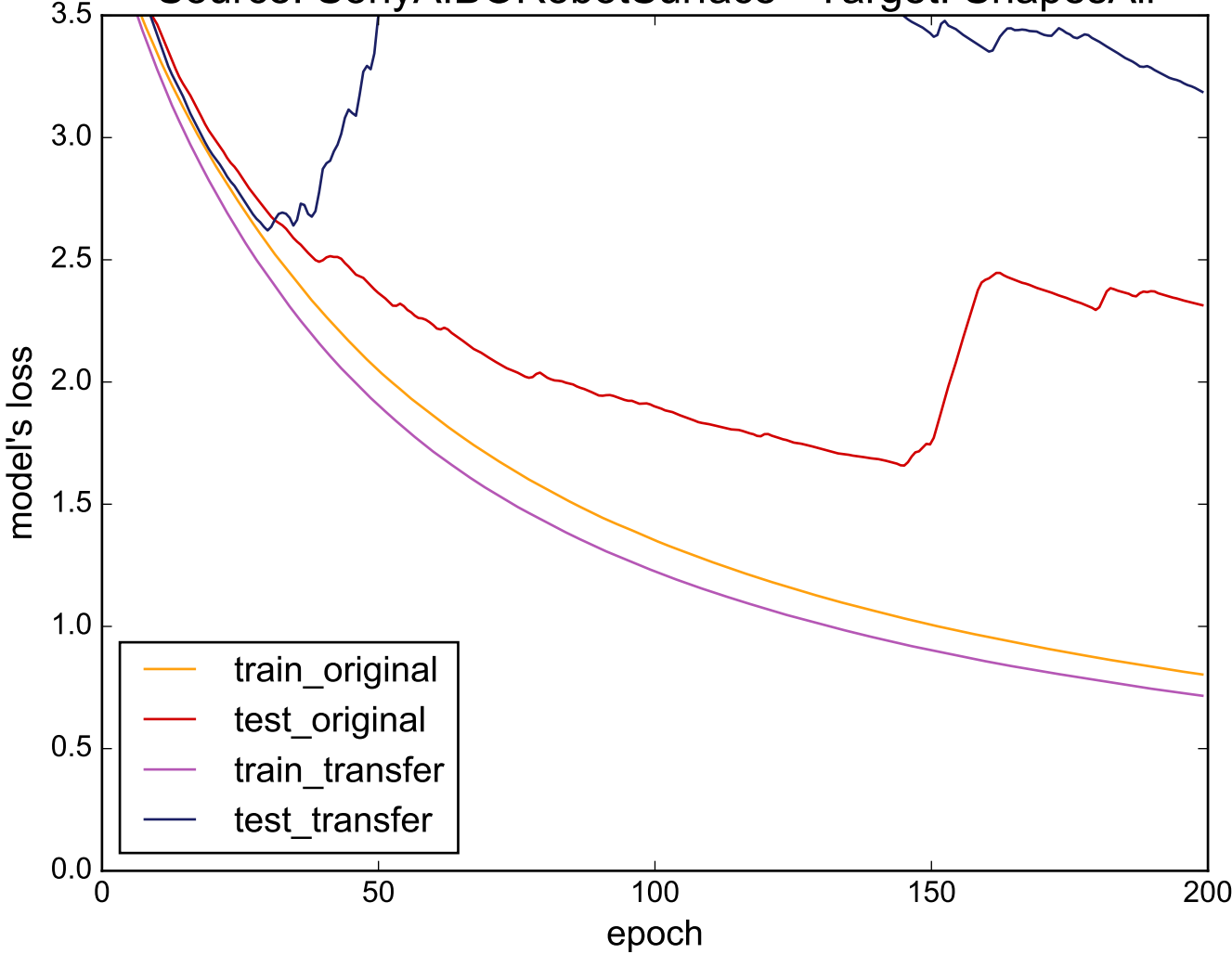
Source: SonyAIBORobotSurface - Target: ShapesAll
