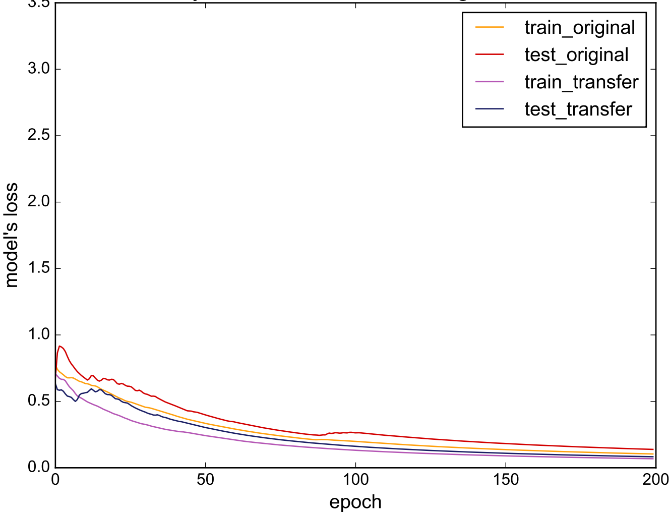
Source: SonyAIBORobotSurface - Target: TwoLeadECG
