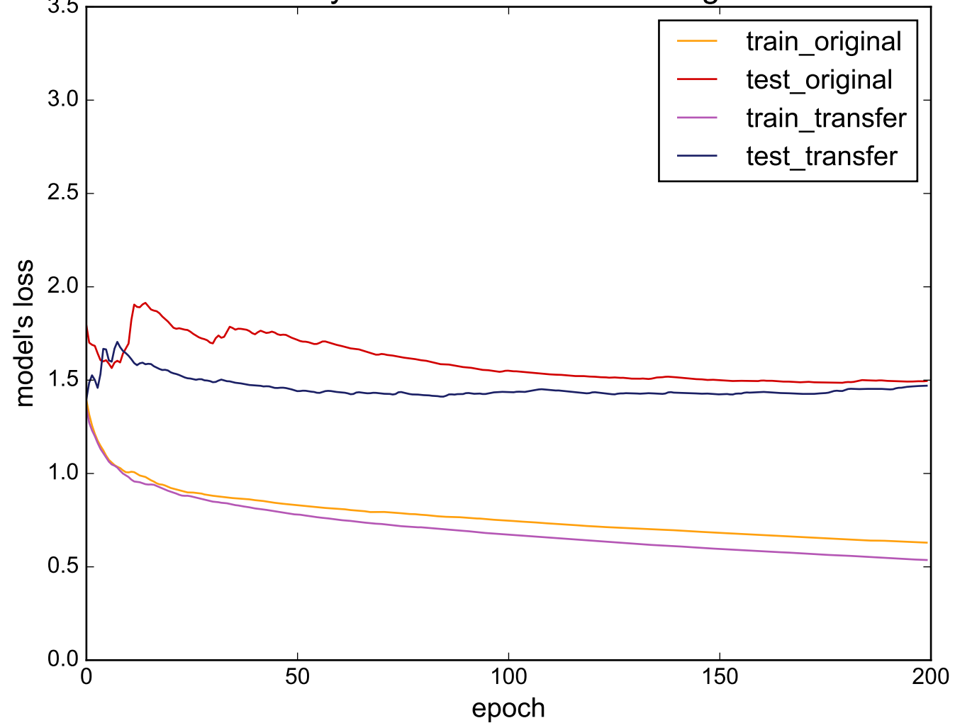
Source: SonyAIBORobotSurface - Target: Worms
