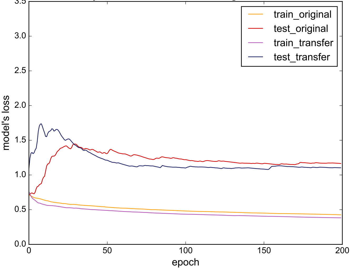
Source: SonyAIBORobotSurface - Target: WormsTwoClass
