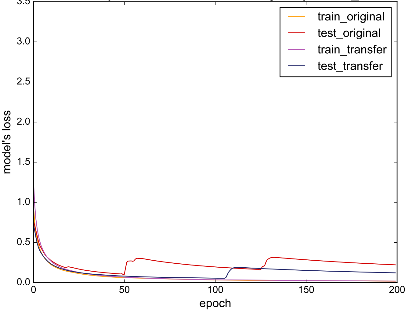
Source: SonyAIBORobotSurface - Target: synthetic_control
