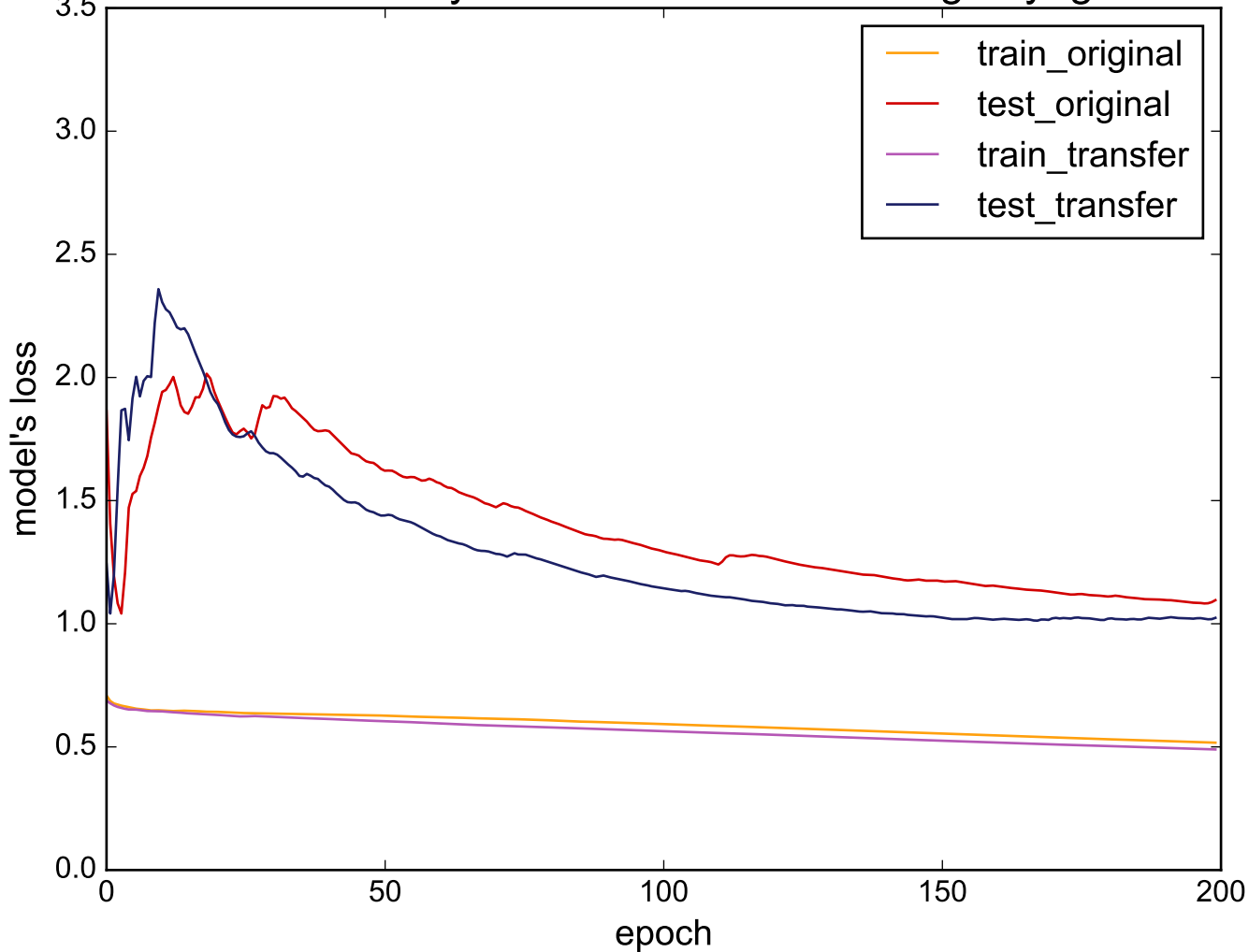
Source: SonyAIBORobotSurface - Target: yoga
