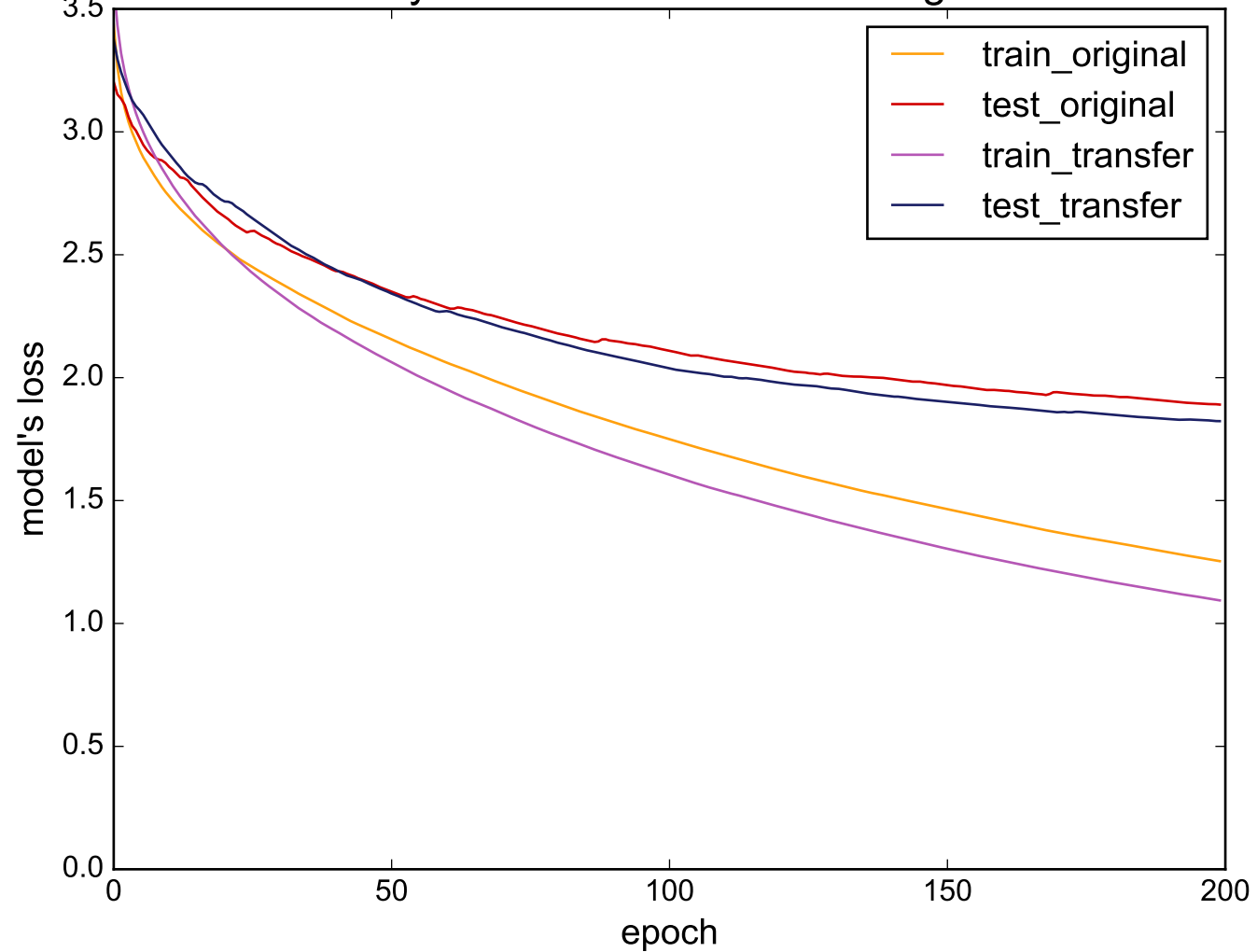
Source: SonyAIBORobotSurfaceII - Target: 50words
