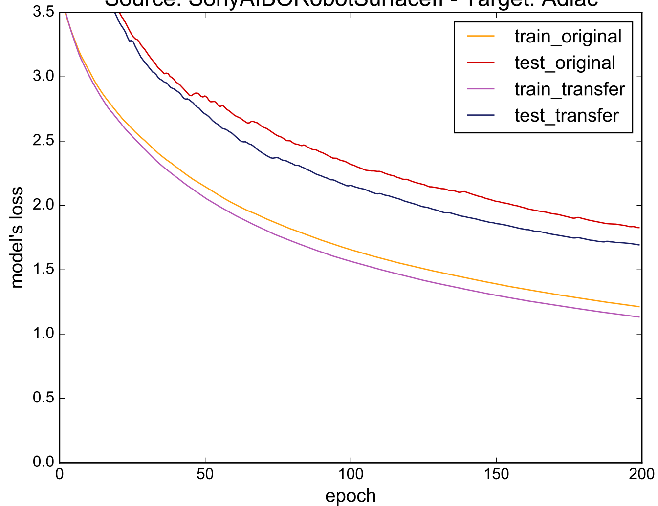
Source: SonyAIBORobotSurfaceII - Target: Adiac
