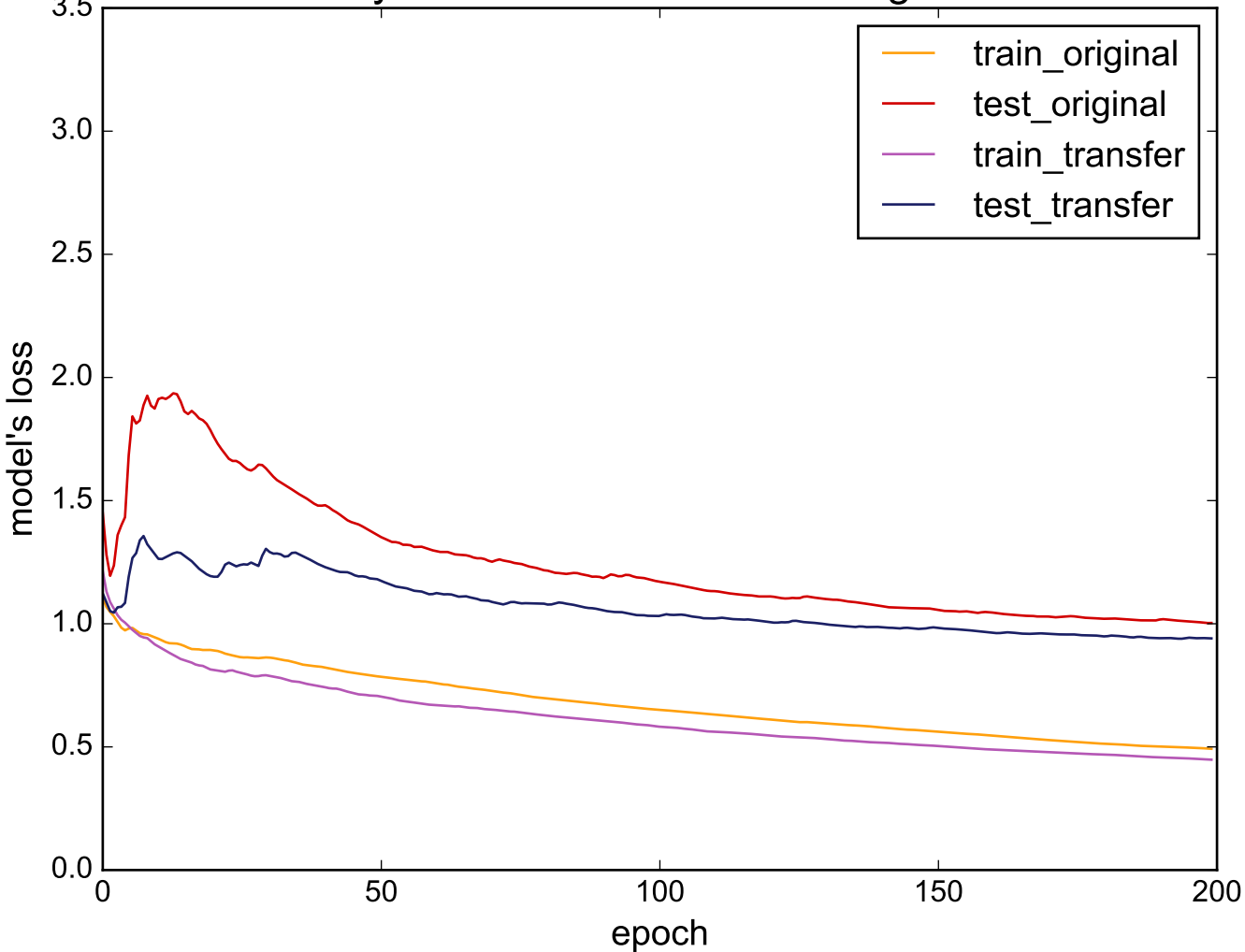
Source: SonyAIBORobotSurfacell - Target: ArrowHead
