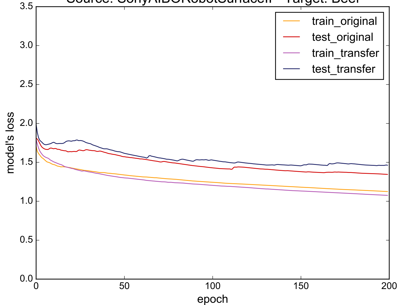
Source: SonyAIBORobotSurfacell - Target: Beef
