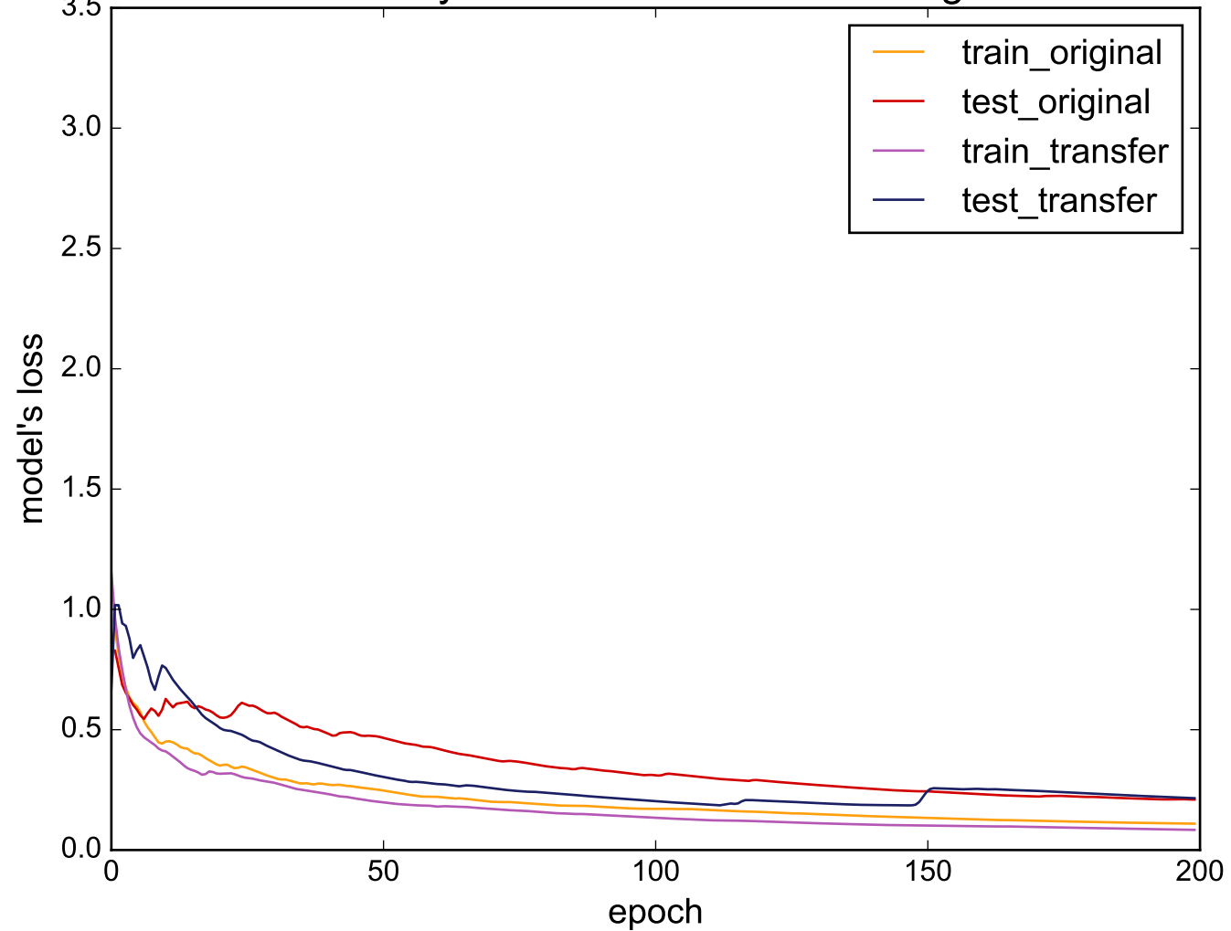
Source: SonyAIBORobotSurfacell - Target: CBF
