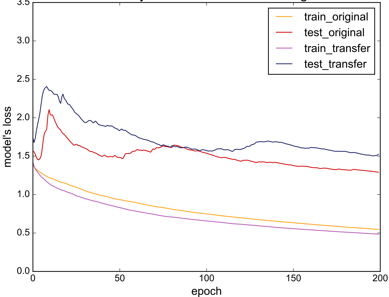
Source: SonyAIBORobotSurfacell - Target: Car
