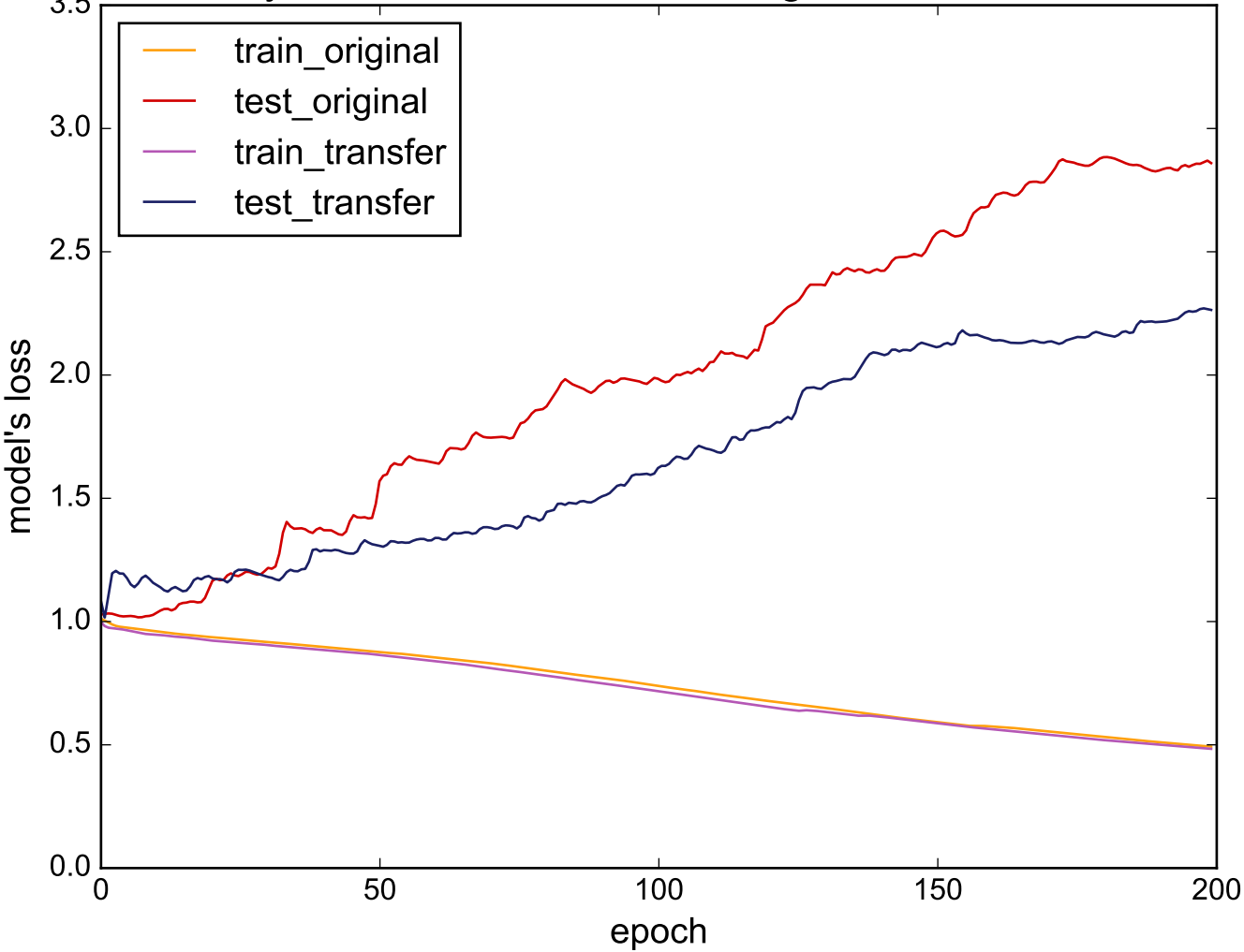
Source: SonyAIBORobotSurfacell - Target: ChlorineConcentration
